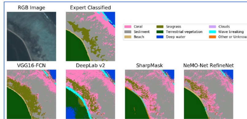
Figure 2: Sample Planet image and classifications. We show comparisons to 3 other popular CNN algorithms besides for NeMO-Net (VGG16, DeepLab, and SharpMask)
